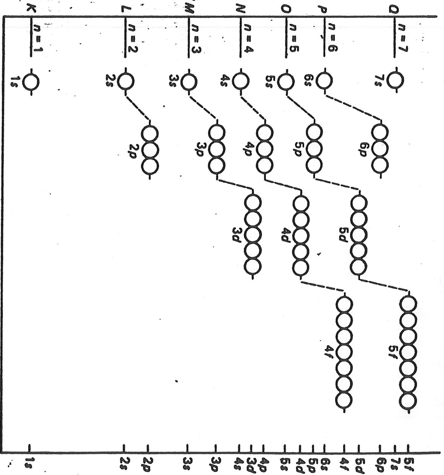
9. Approximate Relative Energy Levels of Subshells
